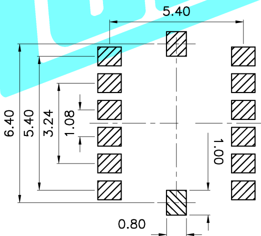
P.C.B Mounting Pattern Dimension
